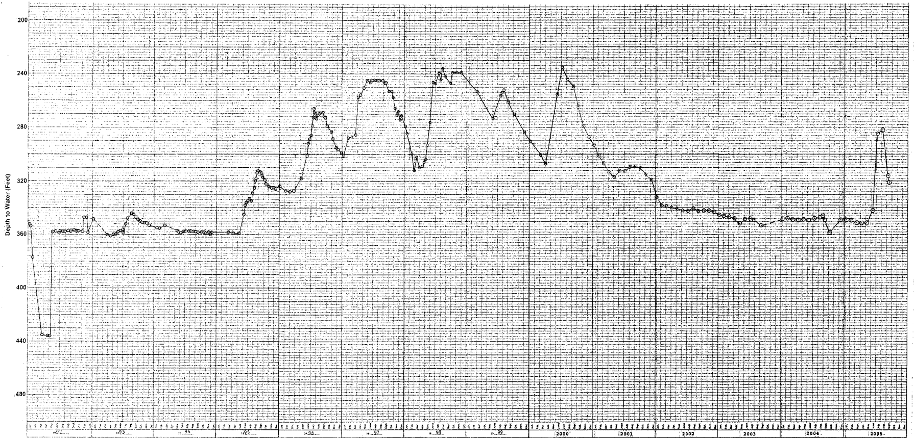
FIGURE 8-WATER-LEVEL HYDROGRAPH FOR WELL NO. 14M
