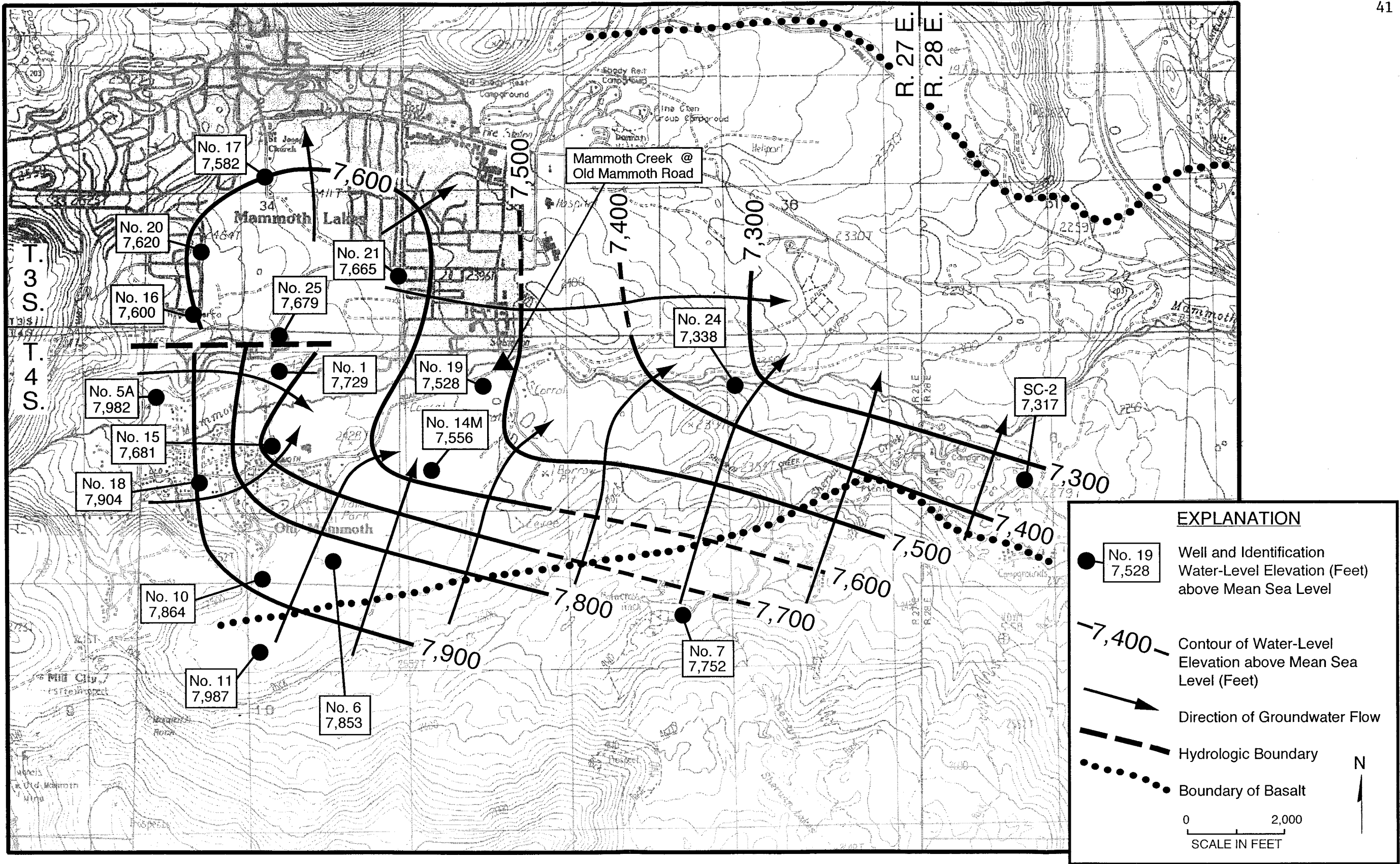
FIGURE 18 - WATER-LEVEL ELEVATIONS IN SEPTEMBER 2005
