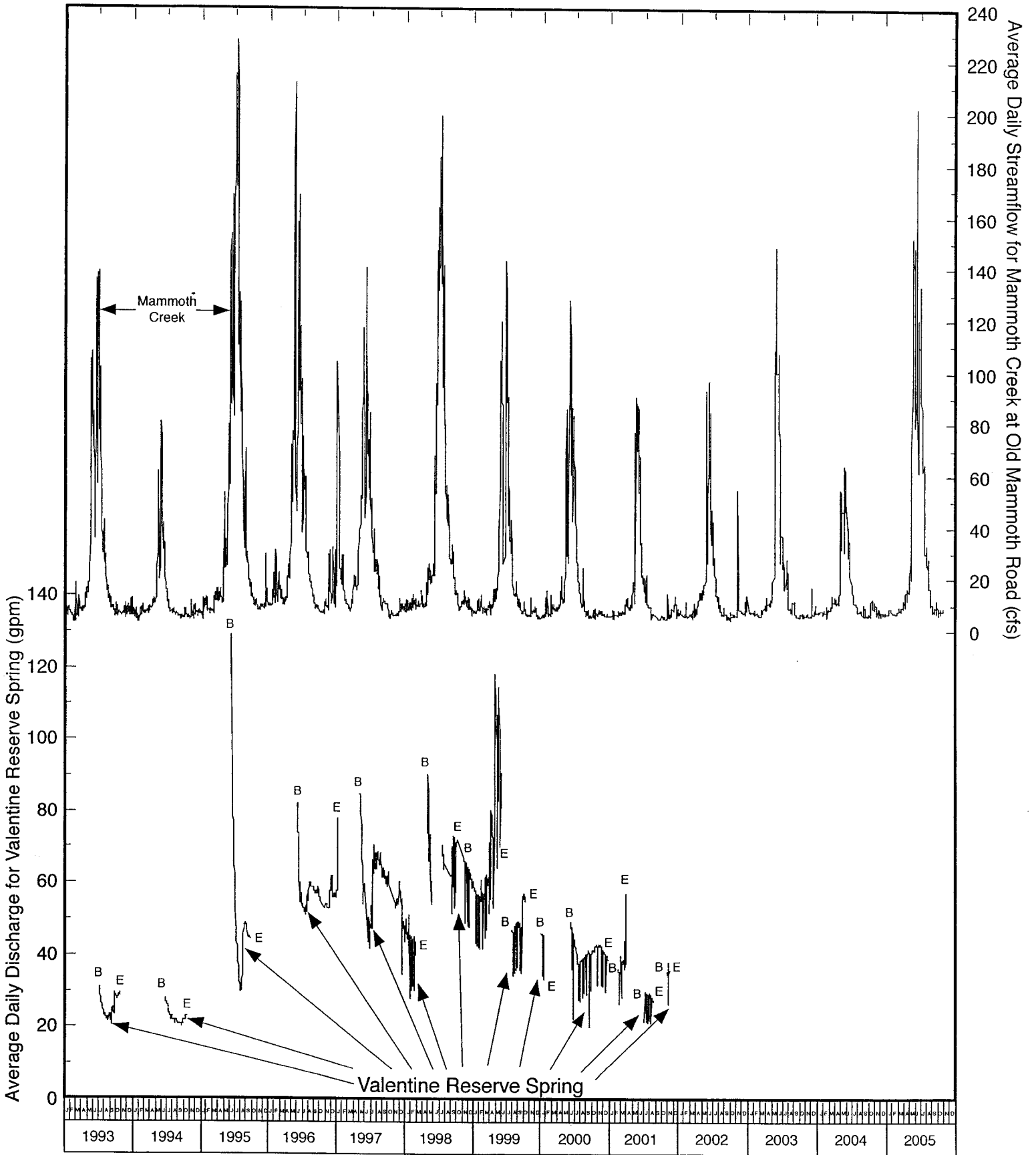
FIGURE 19 - FLOW FOR VALENTINE SPRING (1993-2001) AND MAMMOTH CREEK STREAMFLOW (1993-2005)
