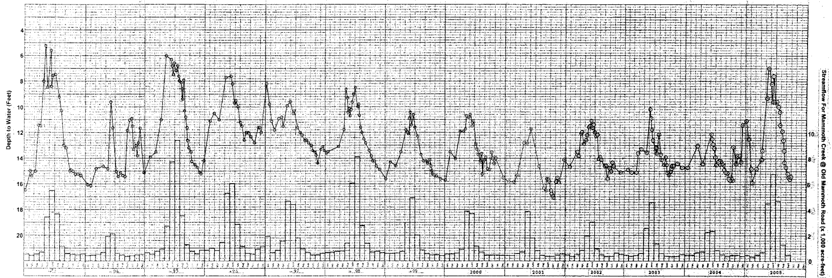
FIGURE 17-WATER-LEVEL HYDROGRAPH FOR WELL NO. 23 AND MAMMOTH CREEK STREAMFLOW
