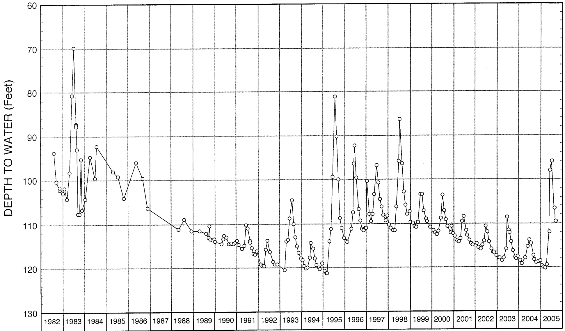
FIGURE 12 - WATER-LEVEL HYDROGRAPH FOR SC-1
