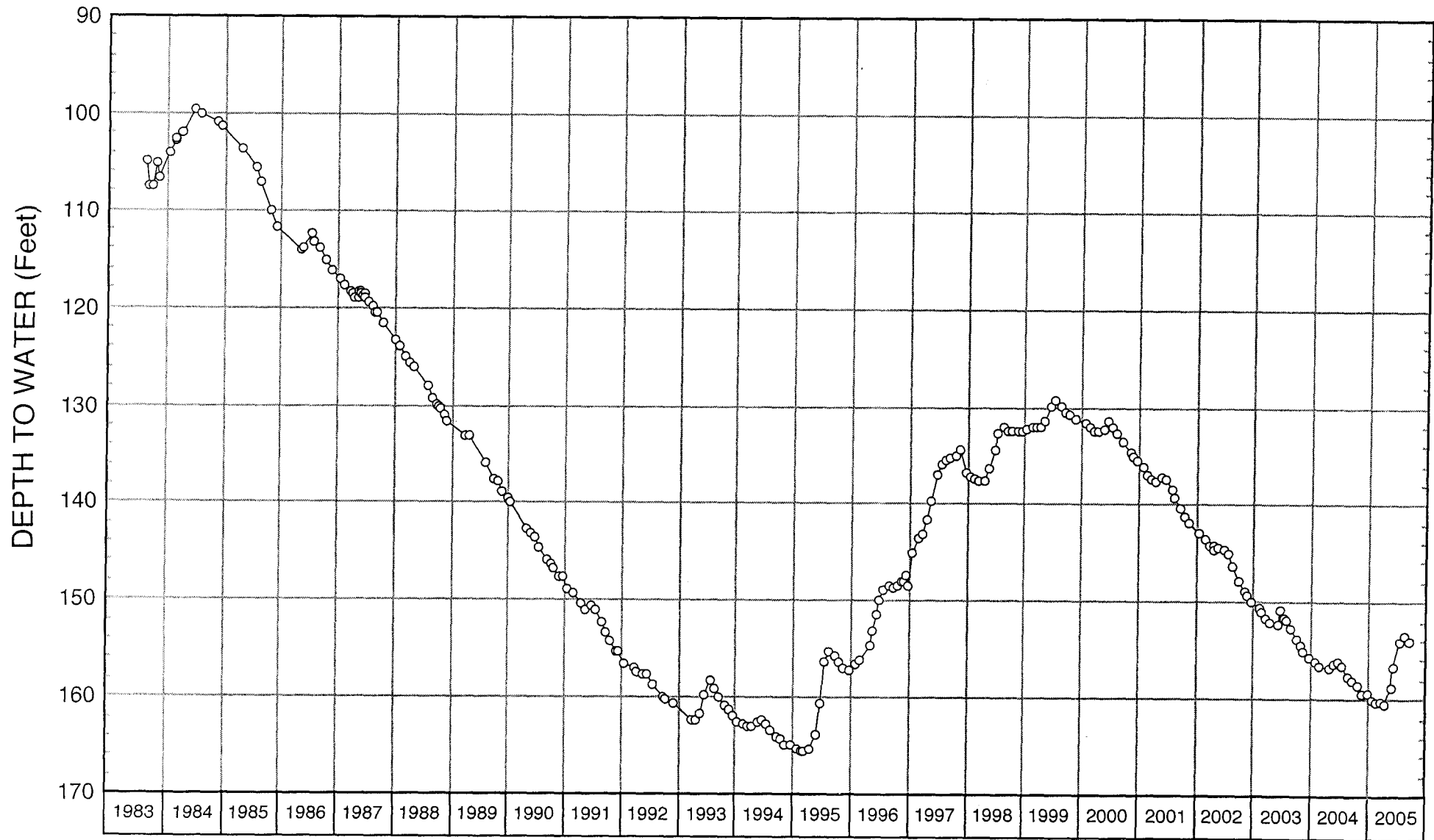
FIGURE 13 - WATER-LEVEL HYDROGRAPH FOR SC-2
